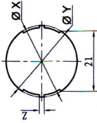
安装孔尺寸 MOUNTING HOLE DIMENTION
